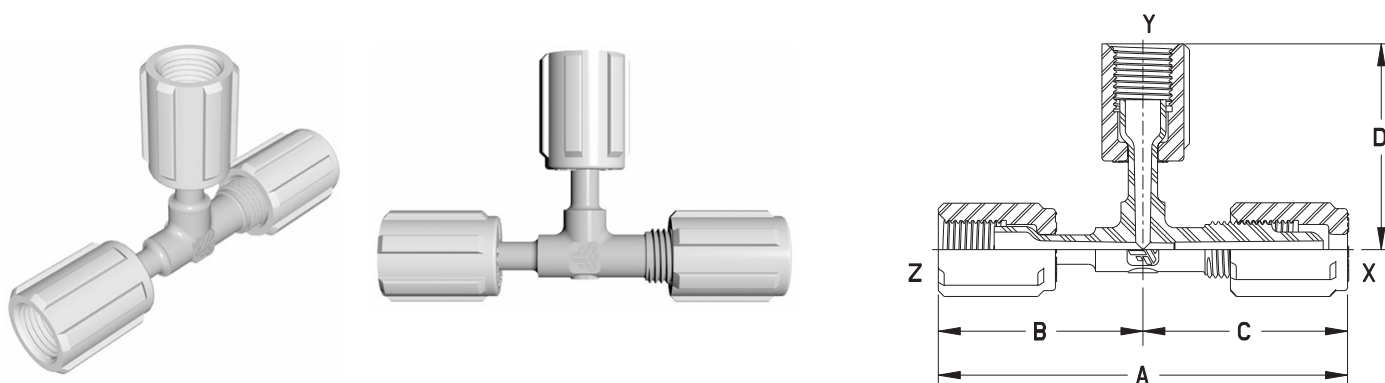
Furon® UTRFF 111 Union Tee Reducer Female Flare 111
