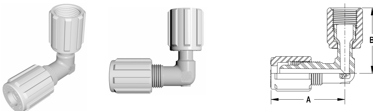
Furon® UEFF Union Elbow Female Flare
