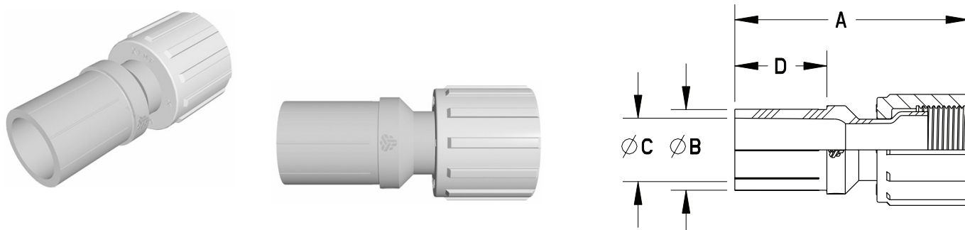
Furon UAFF Union Adapter Female Flare (FuseBond™)
