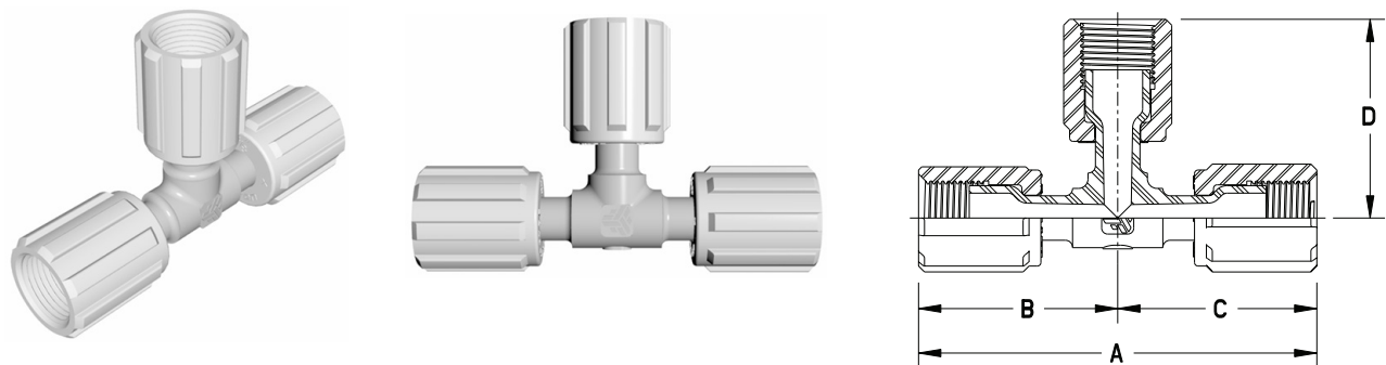
Furon® UTFF 111 Union Tee Female Flare 111
