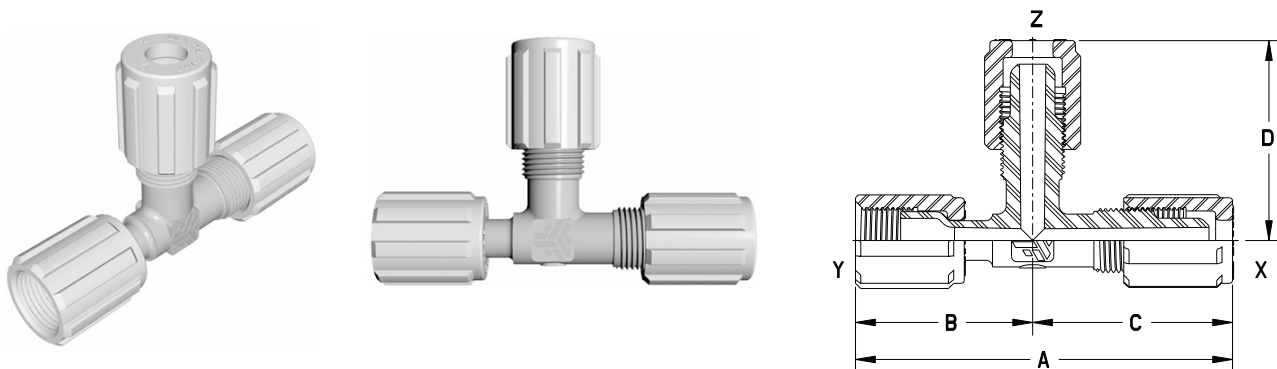
Furon® UTFF I Union Tee Female Flare I
